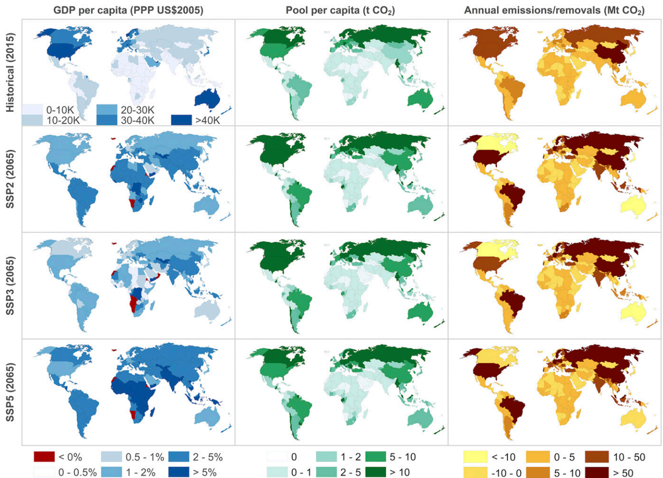
Fig. 2. Spatial patterns in socioeconomic and carbon-pool information for 2015 and projections for 2065. Left shows income per capita, first for 2015 measured in GDP/capita purchasing power parity US$2005 dollars, and then in annual average growth rate from 2015 to 2065 for SSP2, SSP3, and SSP5. Center depicts the relative magnitude of the carbon pool in each country in terms of tCO 2 per capita in 2015 and in 2065 for SSP2, SSP3, and SSP5. Right depicts the annual carbon flux in each country in 2015 and in 2065 for SSP2, SSP3, and SSP5.
